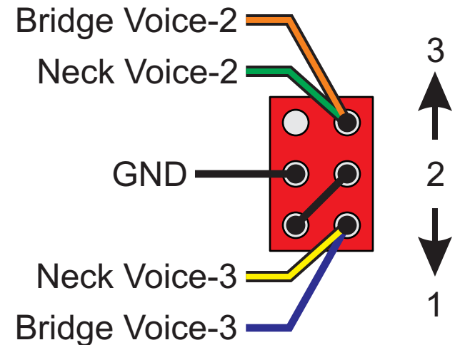
DPDT ON-ON-ON (aka SP3T)
