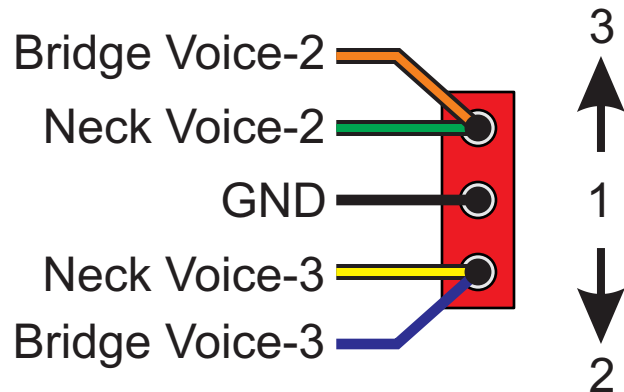
SPDT ON-OFF-ON
